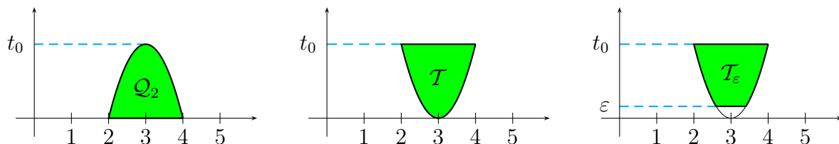
Figure 3: domains \mathcal{Q}_2 , \mathcal{T} , and \mathcal{T}_\varepsilon
